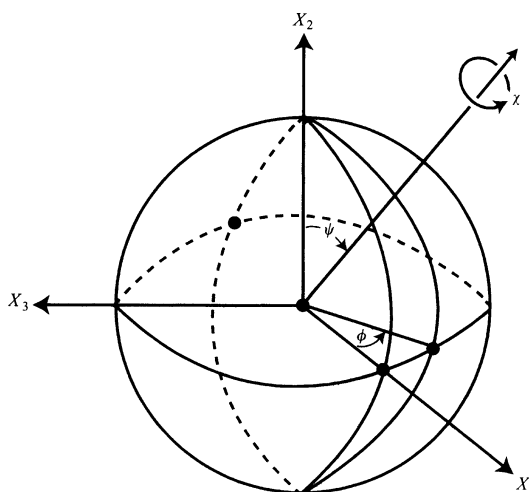
Fig. 10.13 Variables \Psi and \phi are spherical polar coordinates that specify a direction about which the axes may be rotated through an angle \chi
