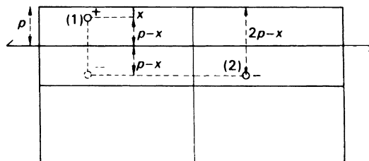
Fig. 2.33 Operation about a 2_1 axis along the line [p, y, 0] : The x coordinate of point 2 relative to that of point 1 is 2p - x . A similar construction may be used for the y coordinate in the c -glide operation
