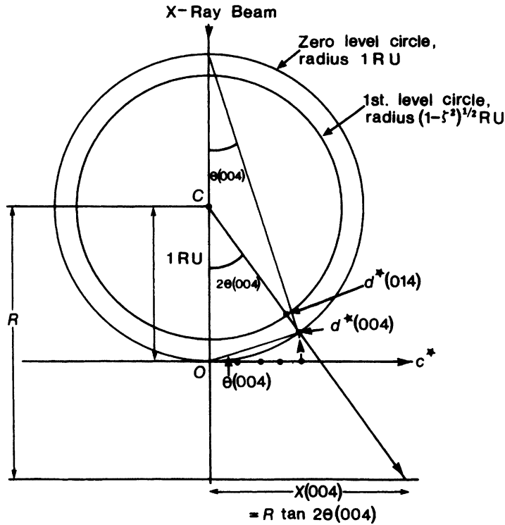
Fig. 5.20 Plan view of flat-plate oscillation geometry, looking down the oscillation axis, CC' in Fig. 5.19, at C. In the accompanying example, the y axis of the crystal (C) is perpendicular to the diagram, and coincides with the rotation axis. Because the crystal is monoclinic, the a^*c^* levels superimpose in this orientation. The diagram shows c^* at the beginning of an anticlockwise rotation perpendicular to the X-ray beam. The crystal rotates through \theta(004) and, at the reciprocal lattice point 004, d^*(004) intersects the Ewald sphere and the 004 reflection is produced. For the 014 reflection, a further small rotation is necessary
