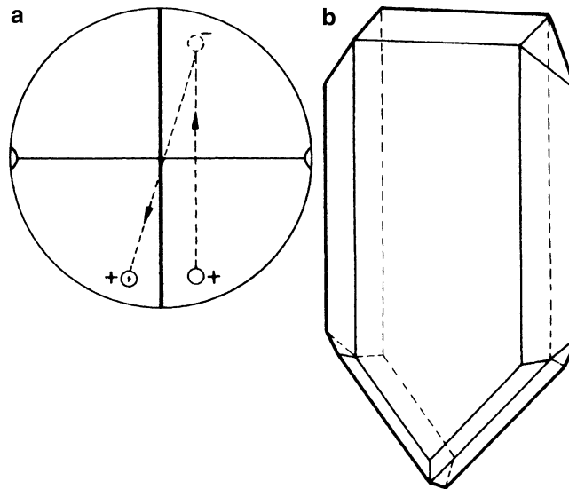
Fig. 1.26 Point group m . (a) Stereogram showing equivalence of m and \bar{2} (the graphic symbol \mathcal{Q} used here for \bar{2} is useful, albeit not conventional). (b) Crystal of potassium tetrathionate ( \text{K}_2\text{S}_4\text{O}_6 ), point group m
