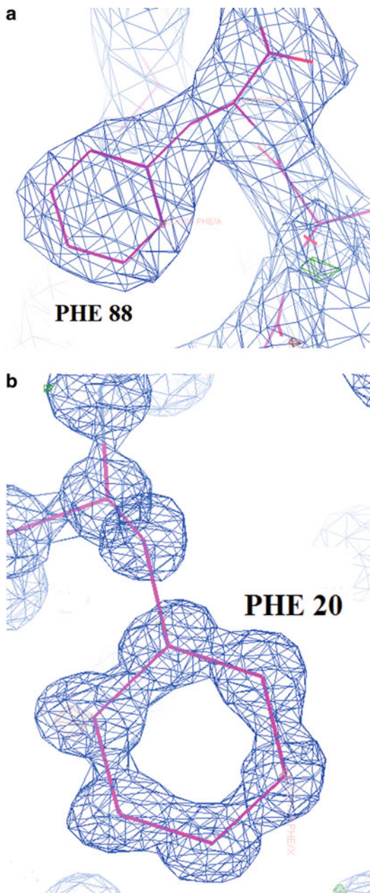
Fig. 10.17 Coot ( 2F_o - |F|_e ) electron density maps. (a) Electron density for mistletoe lectin I (MLI) lactose complex at 2.5 Å resolution in the vicinity of phenylalanine 88 (PHE 88), contoured at the 1.59\sigma level. (b) Bovine ribonuclease A at 0.95 Å in the vicinity of phenylalanine 20 (PHE 20), contoured at the 1.6\sigma level: \sigma is the rms deviation of the average electron density, a quantitative way of assessing the noise level of the map. The choice of contour levels determines both the appearance of the output map and the ease of interpretation. The effect of resolution is clearly apparent emphasizing the need for a program like Coot, which assigns coordinates to the model atoms in such a way as to preserve the molecular geometry. Assignment of atomic coordinates is obviously much easier for the higher resolution map (b) (Coot maps provided by courtesy of Dr. David Lisgarten)
