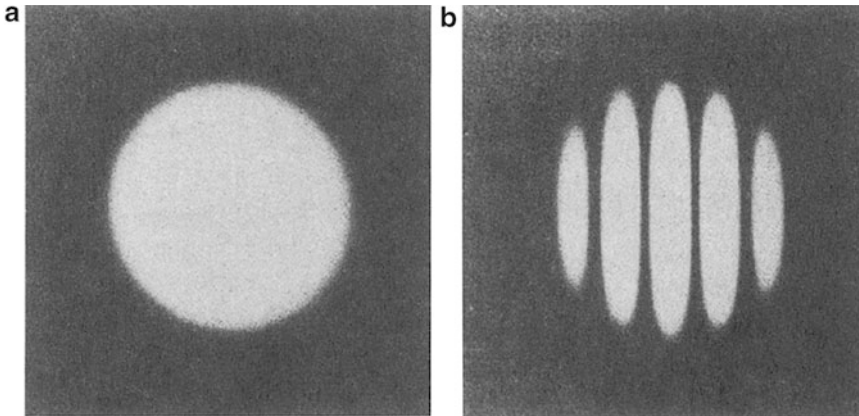
Fig. 6.9 Diffraction patterns from circular holes. (a) One hole 1 mm diameter. (b) Two holes each of 1 mm diameter, set 3 mm apart in the horizontal direction (reproduced from Taylor and Lipson 1964)
